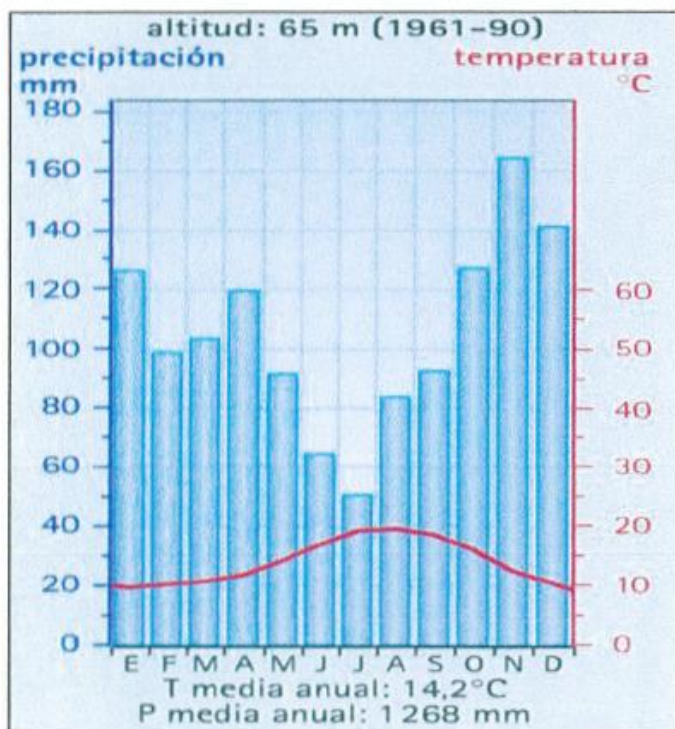
CLIMOGRAMA A
