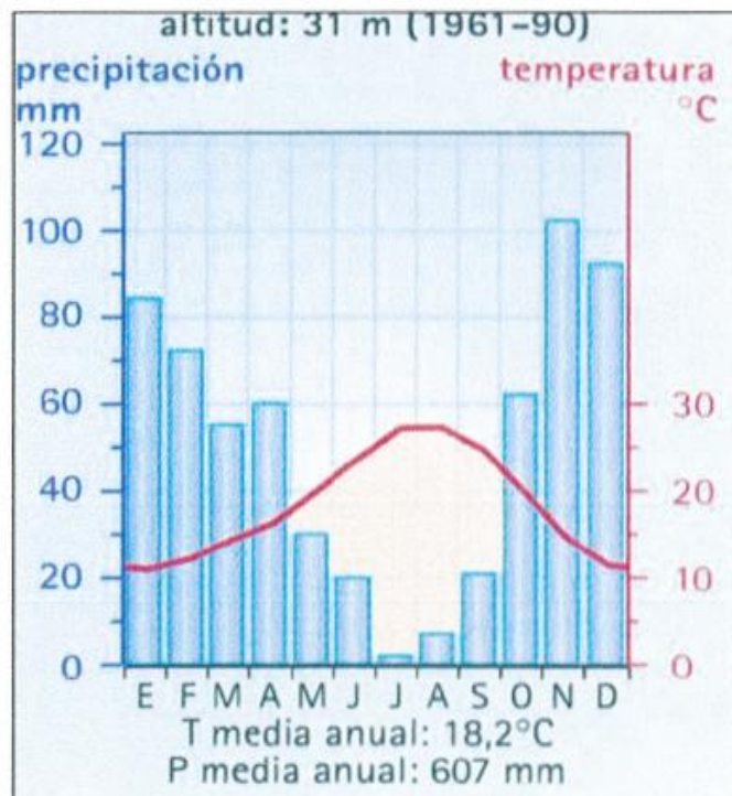
CLIMOGRAMA B
