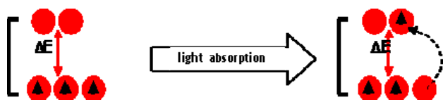
Figure 3. Scheme of a d-d transition for Cr(III) in an octahedral field
