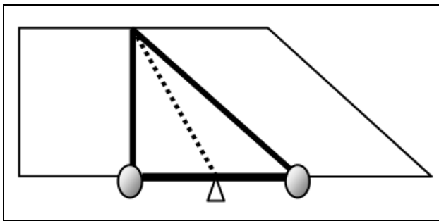
Figure 22. Galilean transformation
