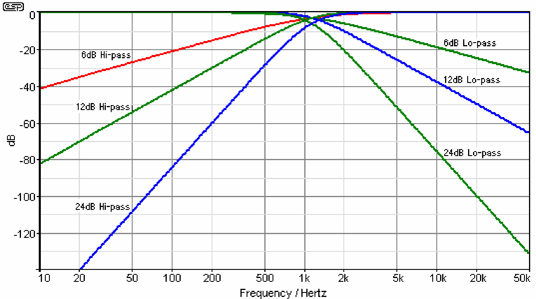
Typical Filter Slopes
