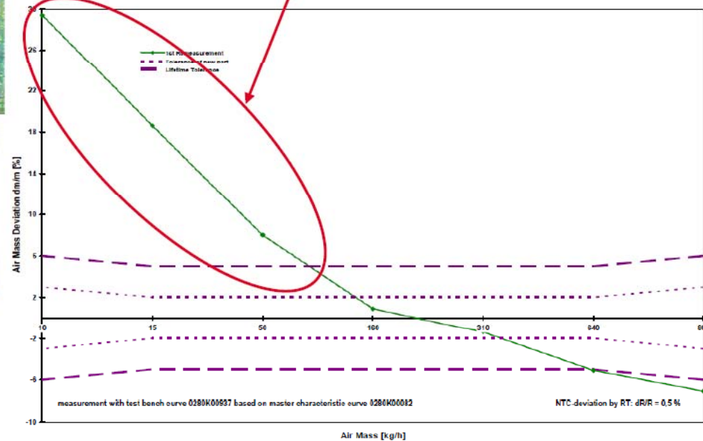
Measurement with Characteristic Curve of KD-2770
