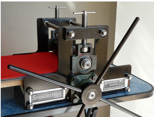
PRINTING PRESS
